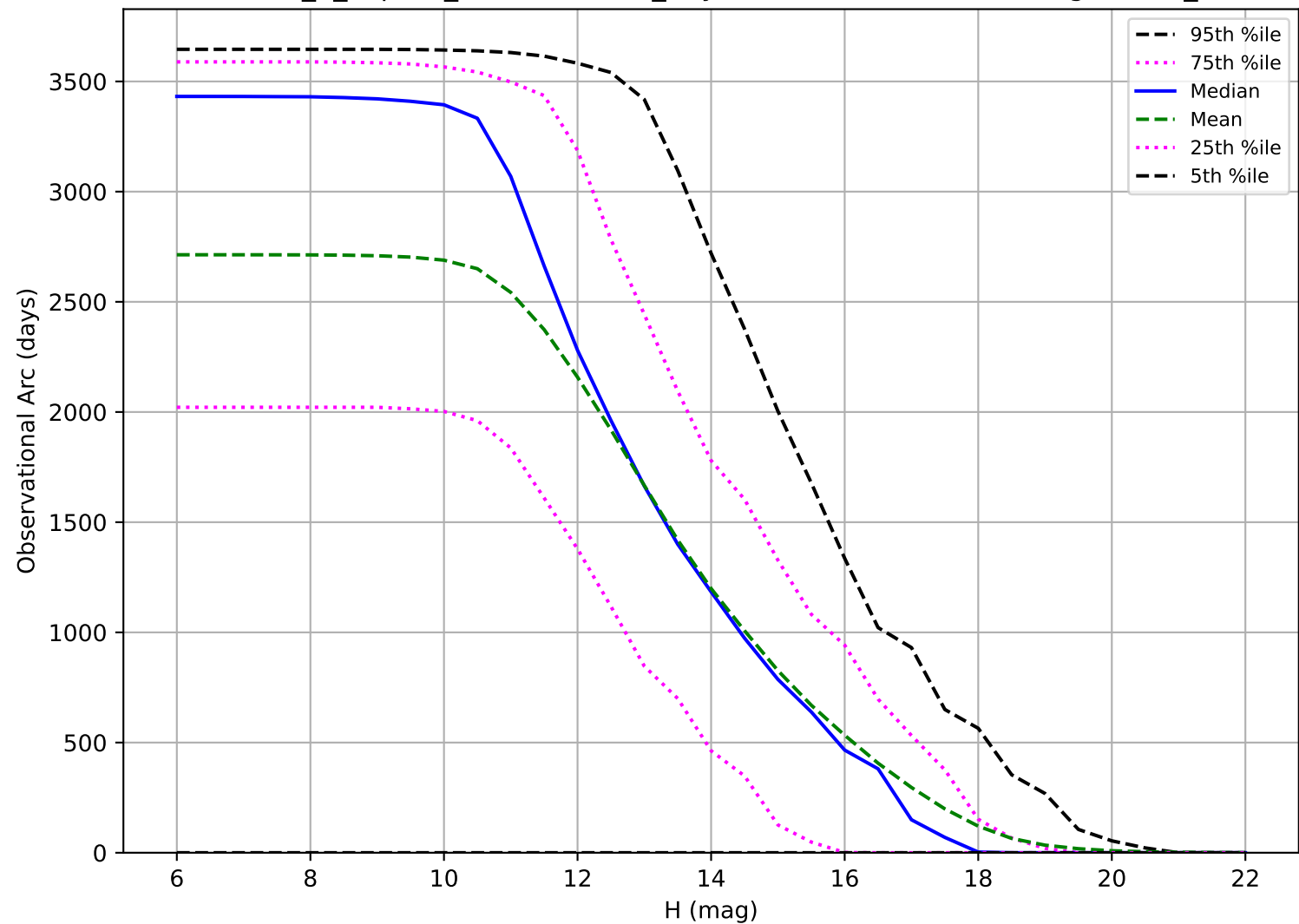
internal_u_expt38_nscale0.9v3.4_10yrs: Observational Arc Length OCC_r5
