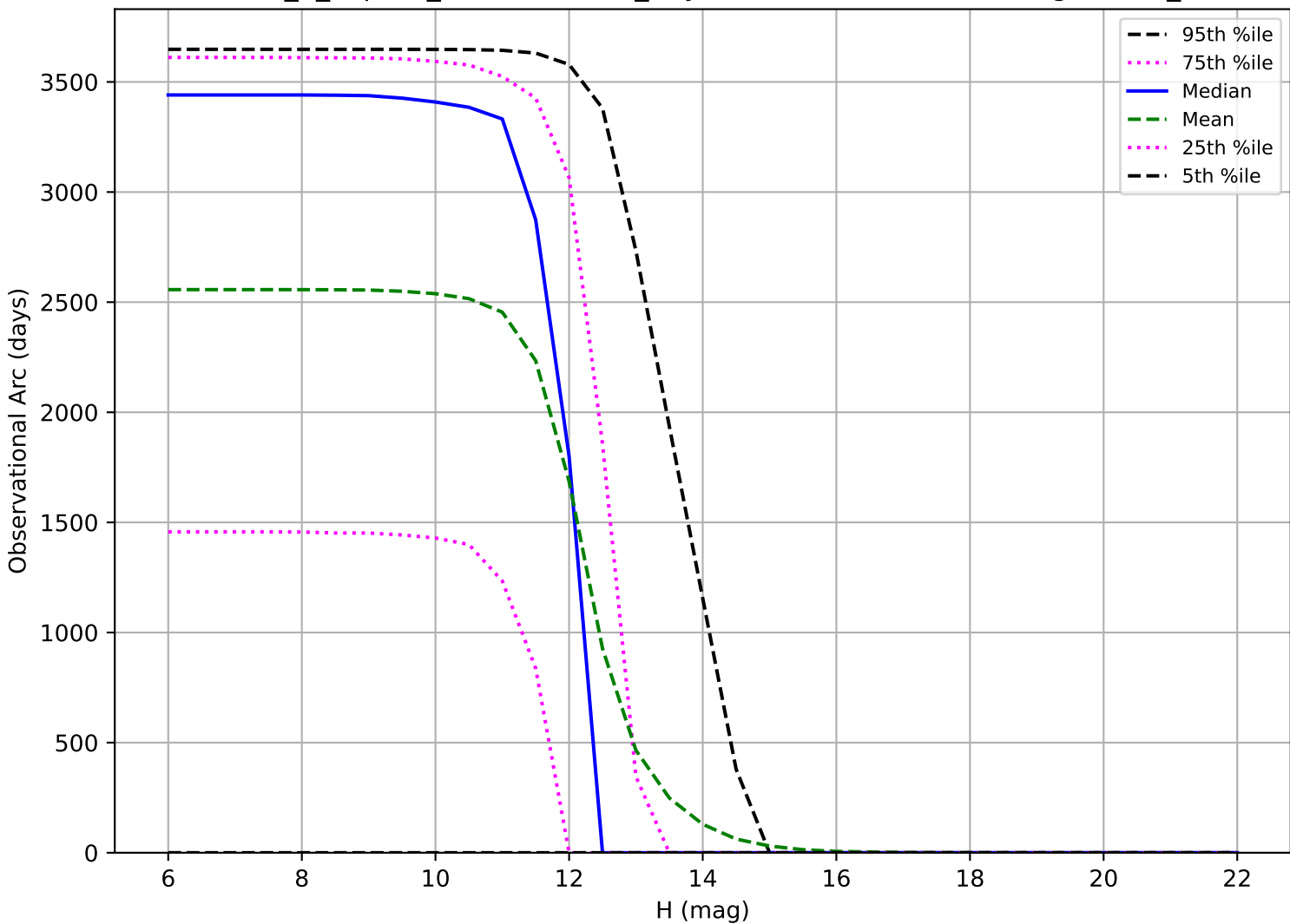
internal_u_expt38_nscale0.9v3.4_10yrs: Observational Arc Length OCC_r20
