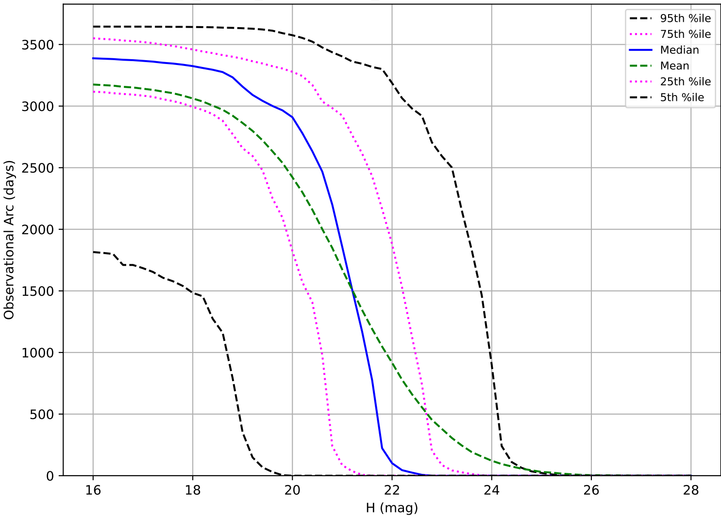
internal_u_expt38_nscale0.9v3.4_10yrs: Observational Arc Length NEO
