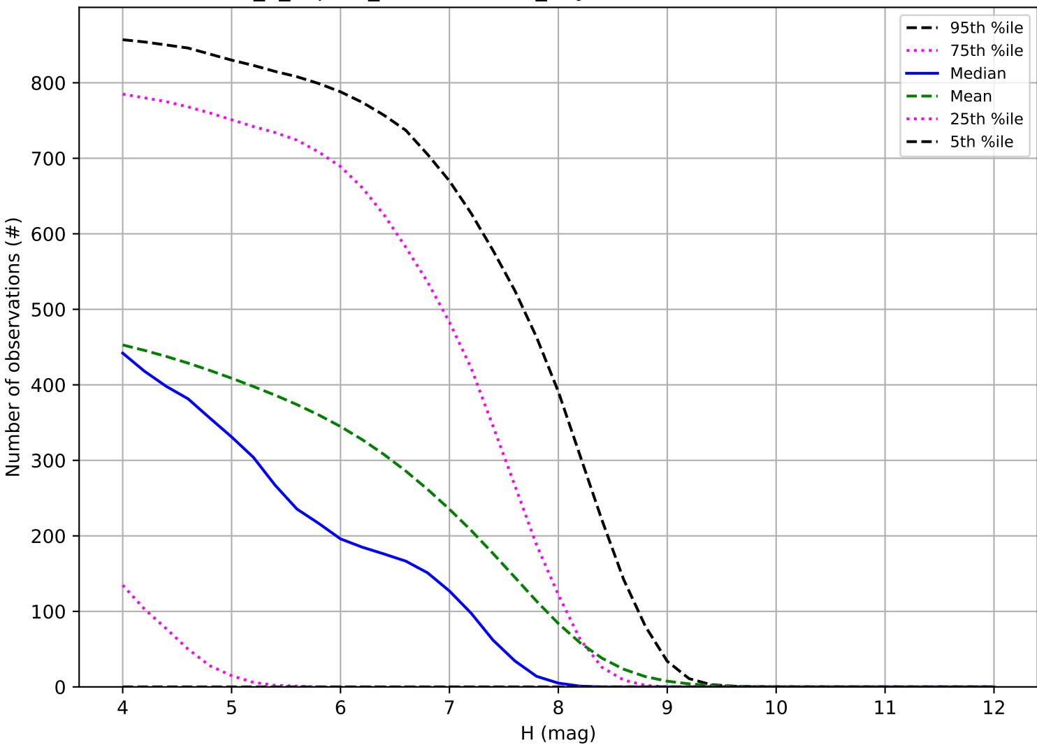
internal_u_expt38_nscale0.9v3.4_10yrs: Number of observations TNO
