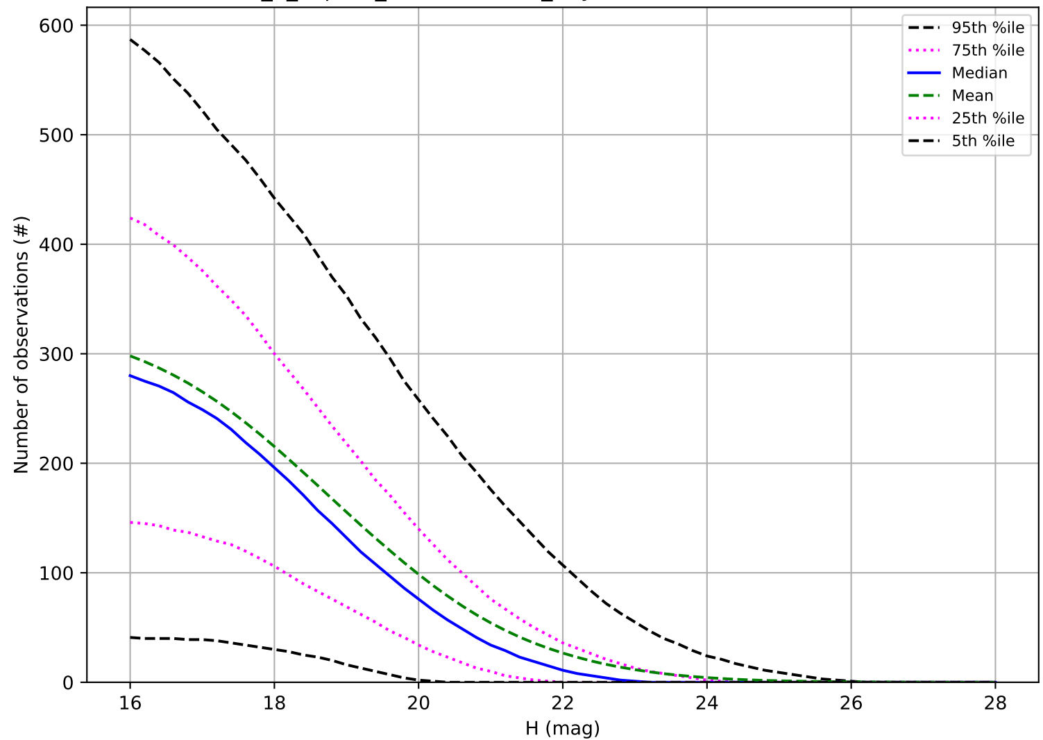
internal_u_expt38_nscale0.9v3.4_10yrs: Number of observations PHA
