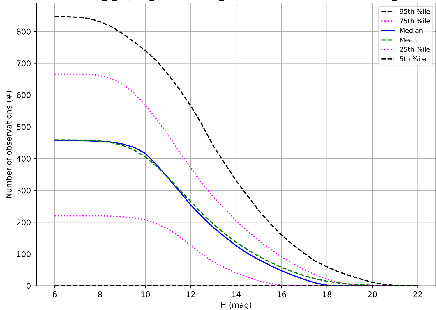
internal_u_expt38_nscale0.9v3.4_10yrs: Number of observations OCC_r5
