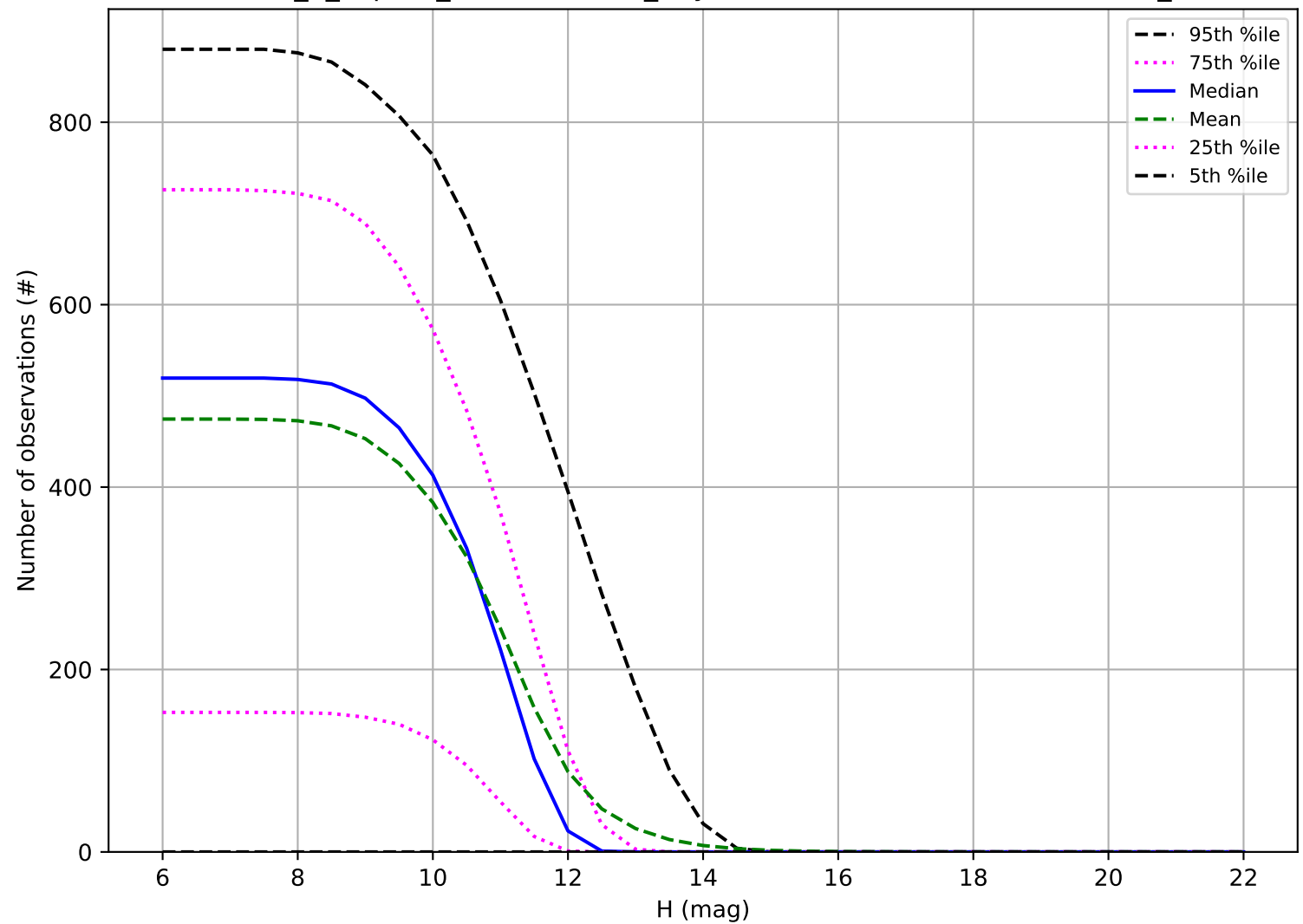
internal_u_expt38_nscale0.9v3.4_10yrs: Number of observations OCC_r20
