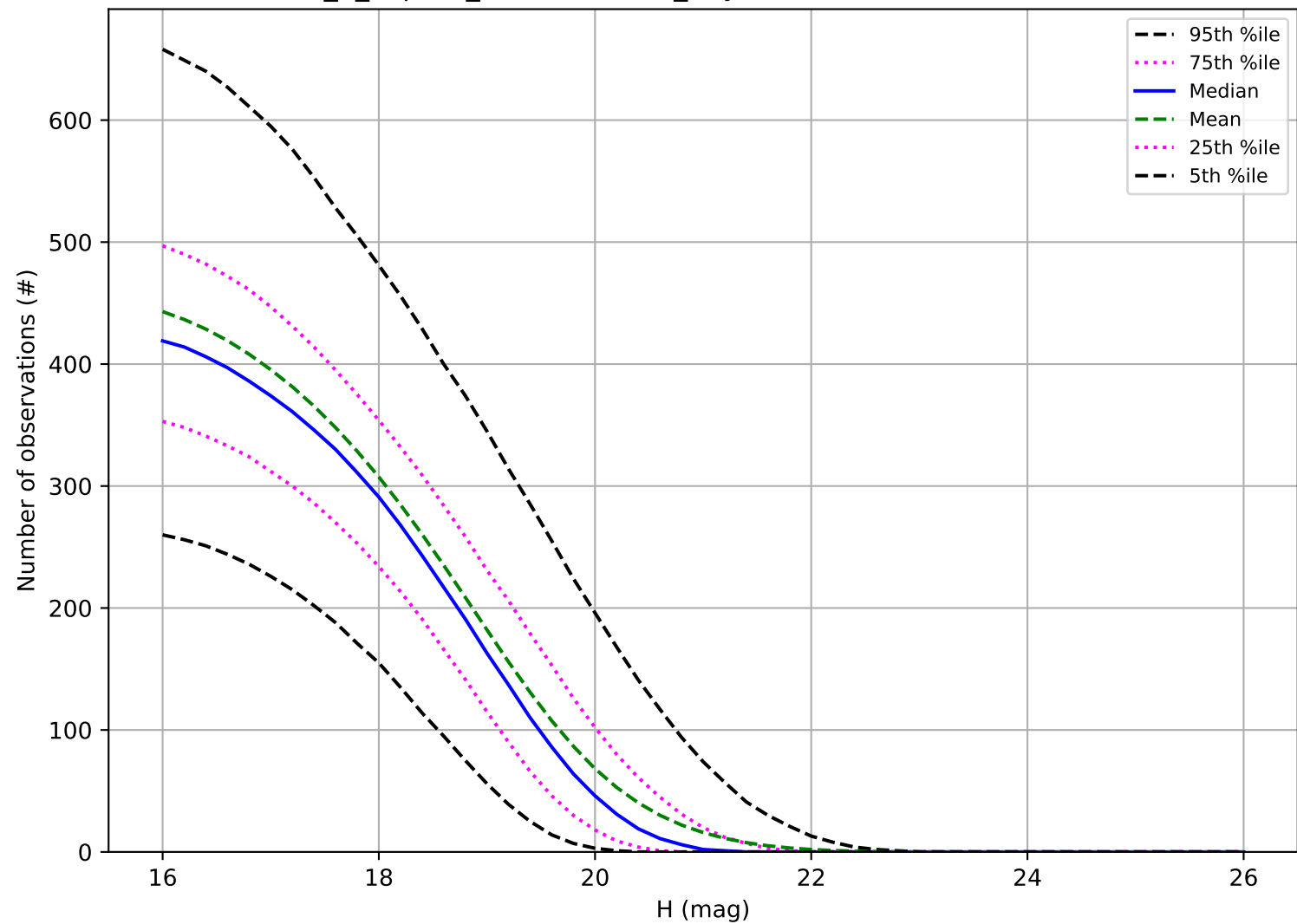
internal_u_expt38_nscale0.9v3.4_10yrs: Number of observations MBA
