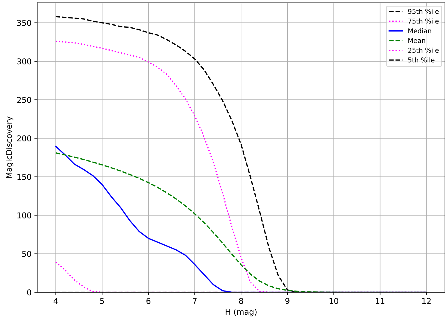
internal_u_expt38_nscale0.9v3.4_10yrs: TNO 6 detections in 60 nights detection loss
