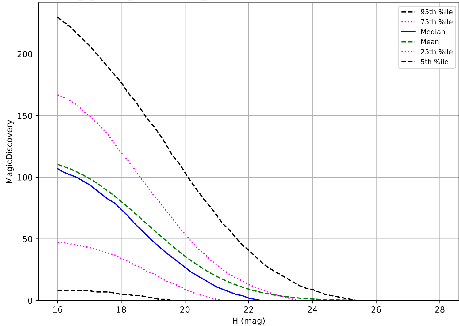
internal_u_expt38_nscale0.9v3.4_10yrs: PHA 6 detections in 60 nights detection loss
