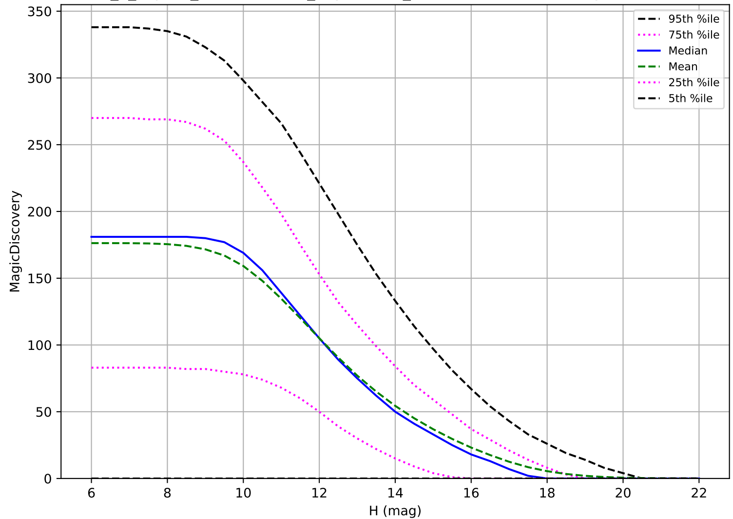
internal_u_expt38_nscale0.9v3.4_10yrs: OCC_r5 6 detections in 60 nights detection loss
