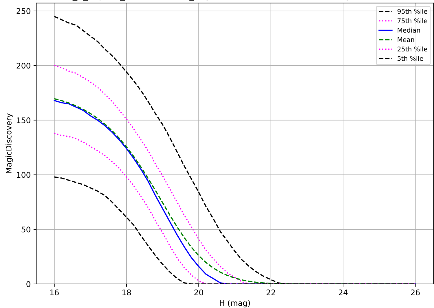
internal_u_expt38_nscale0.9v3.4_10yrs: MBA 6 detections in 60 nights detection loss
