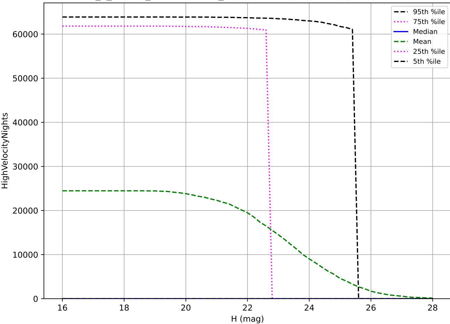
internal_u_expt38_nscale0.9v3.4_10yrs: PHA High velocity pair detection loss
