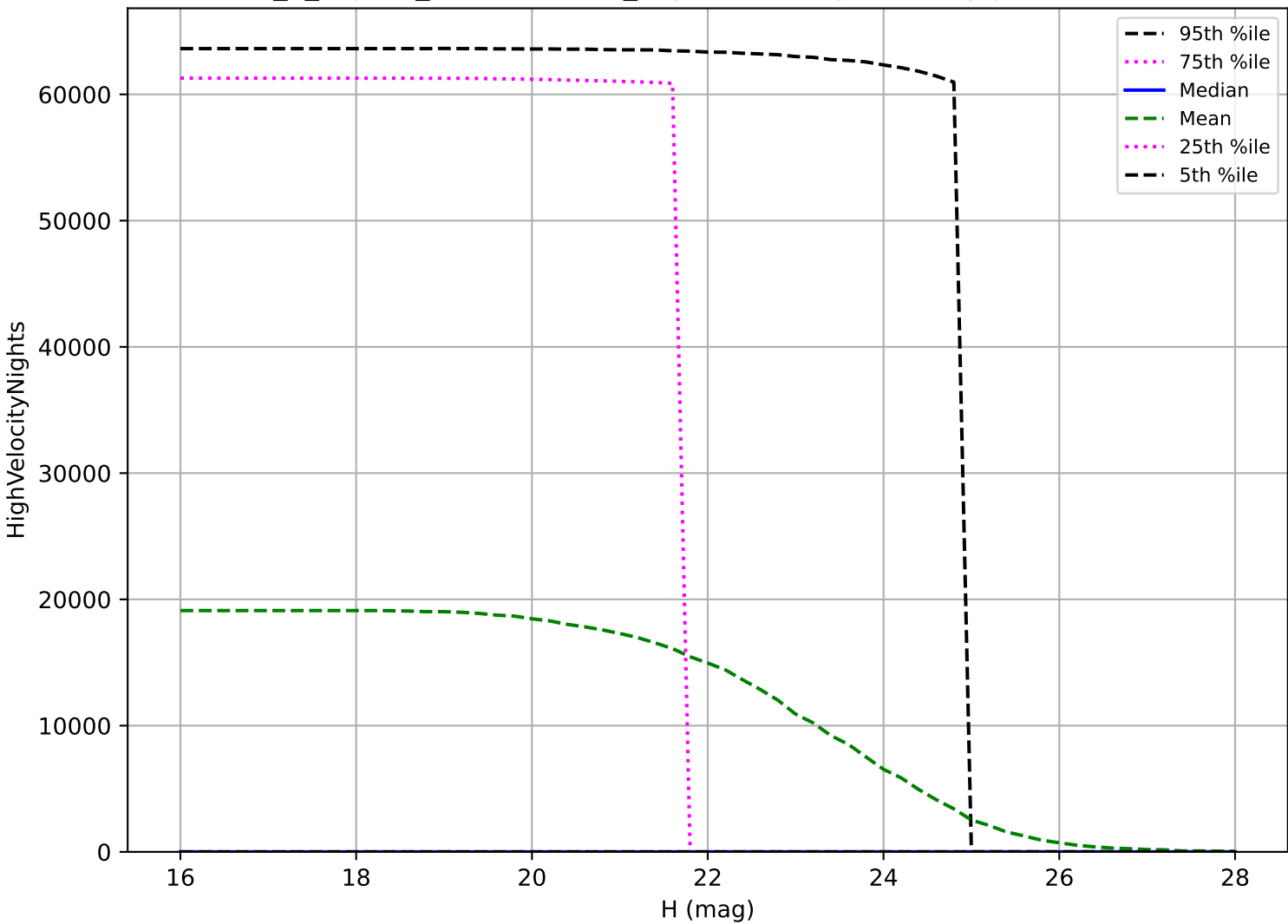
internal_u_expt38_nscale0.9v3.4_10yrs: NEO High velocity pair detection loss
