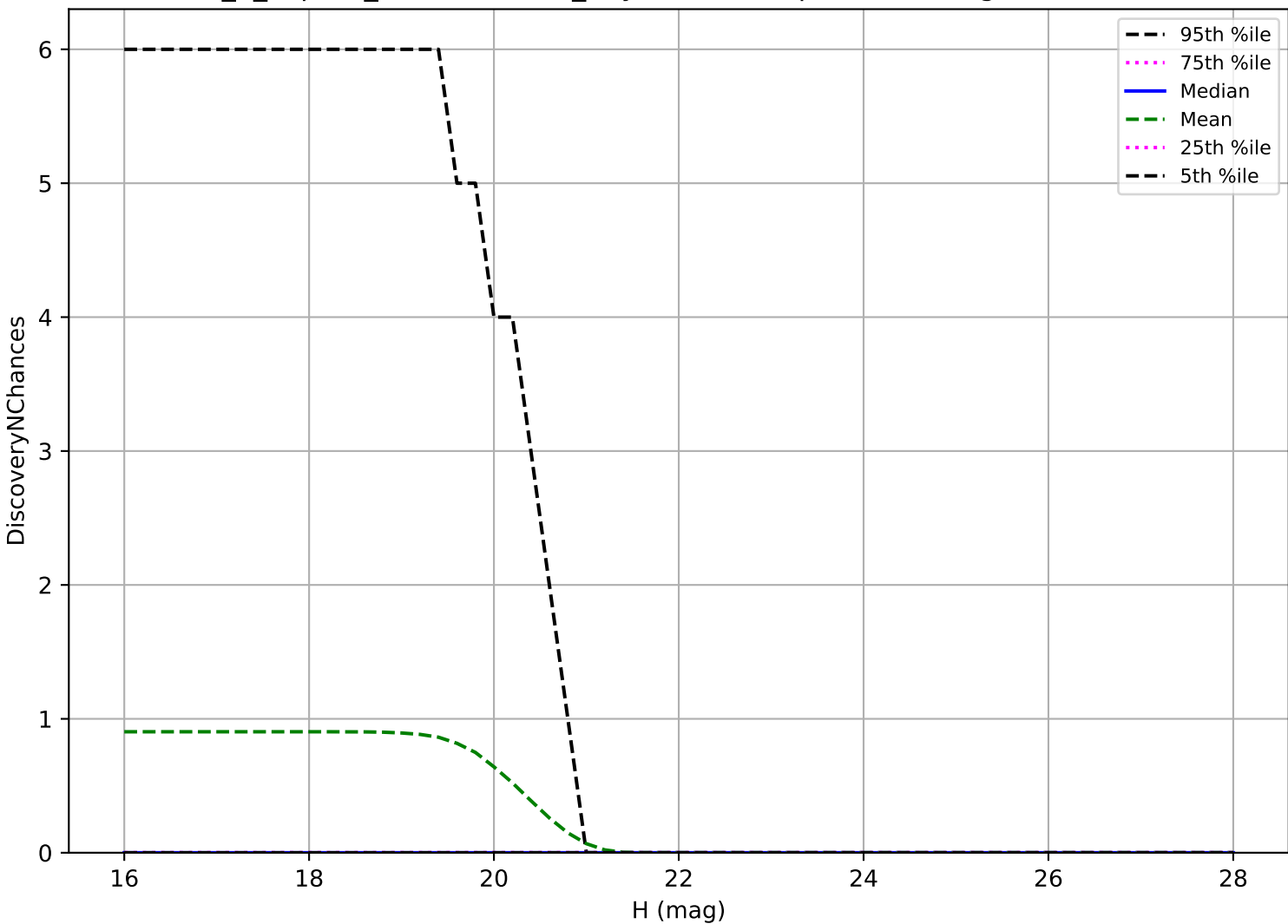
internal_u_expt38_nscale0.9v3.4_10yrs: Vatira 3 pairs in 15 nights detection loss
