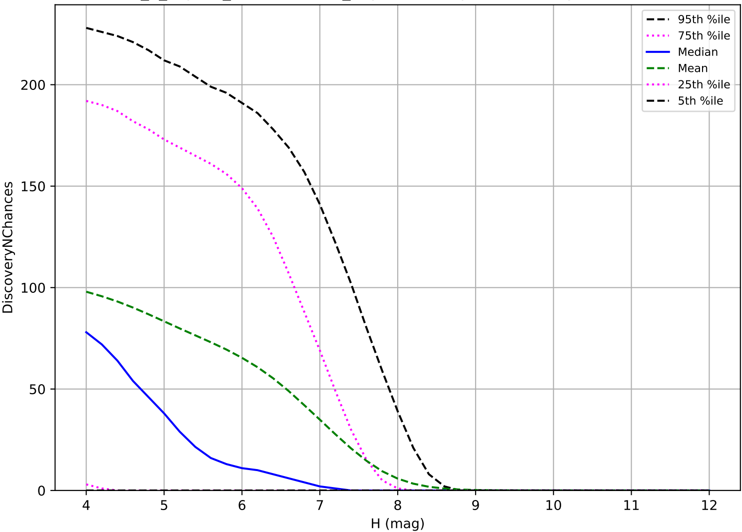
internal_u_expt38_nscale0.9v3.4_10yrs: TNO 3 pairs in 15 nights detection loss
