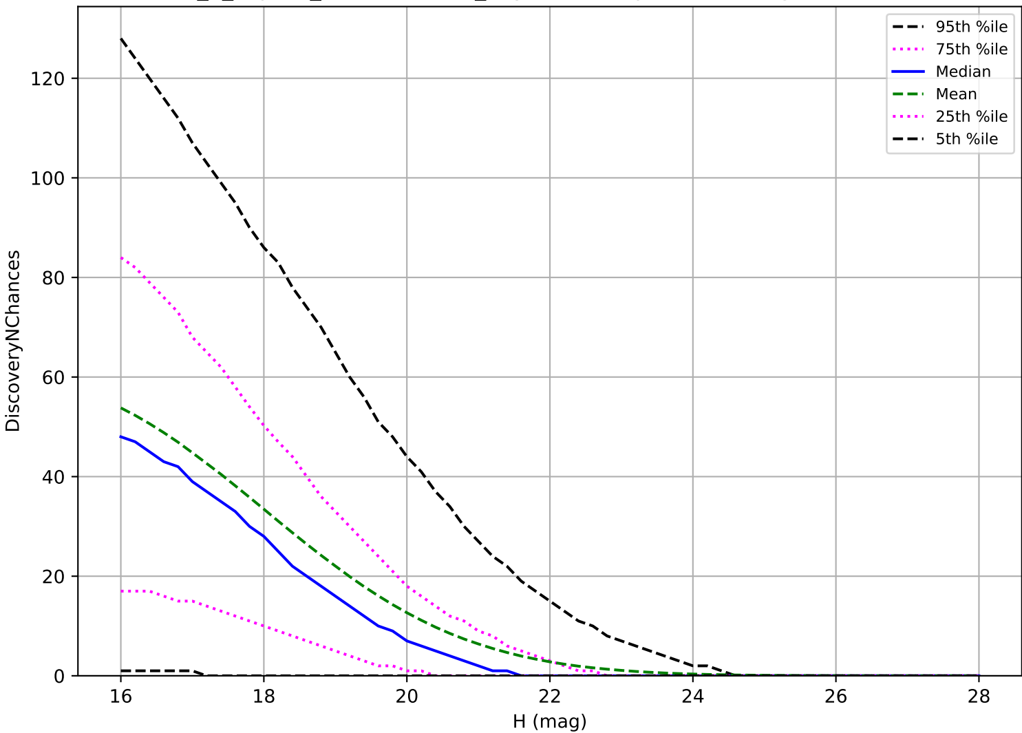
internal_u_expt38_nscale0.9v3.4_10yrs: PHA 3 pairs in 15 nights detection loss
