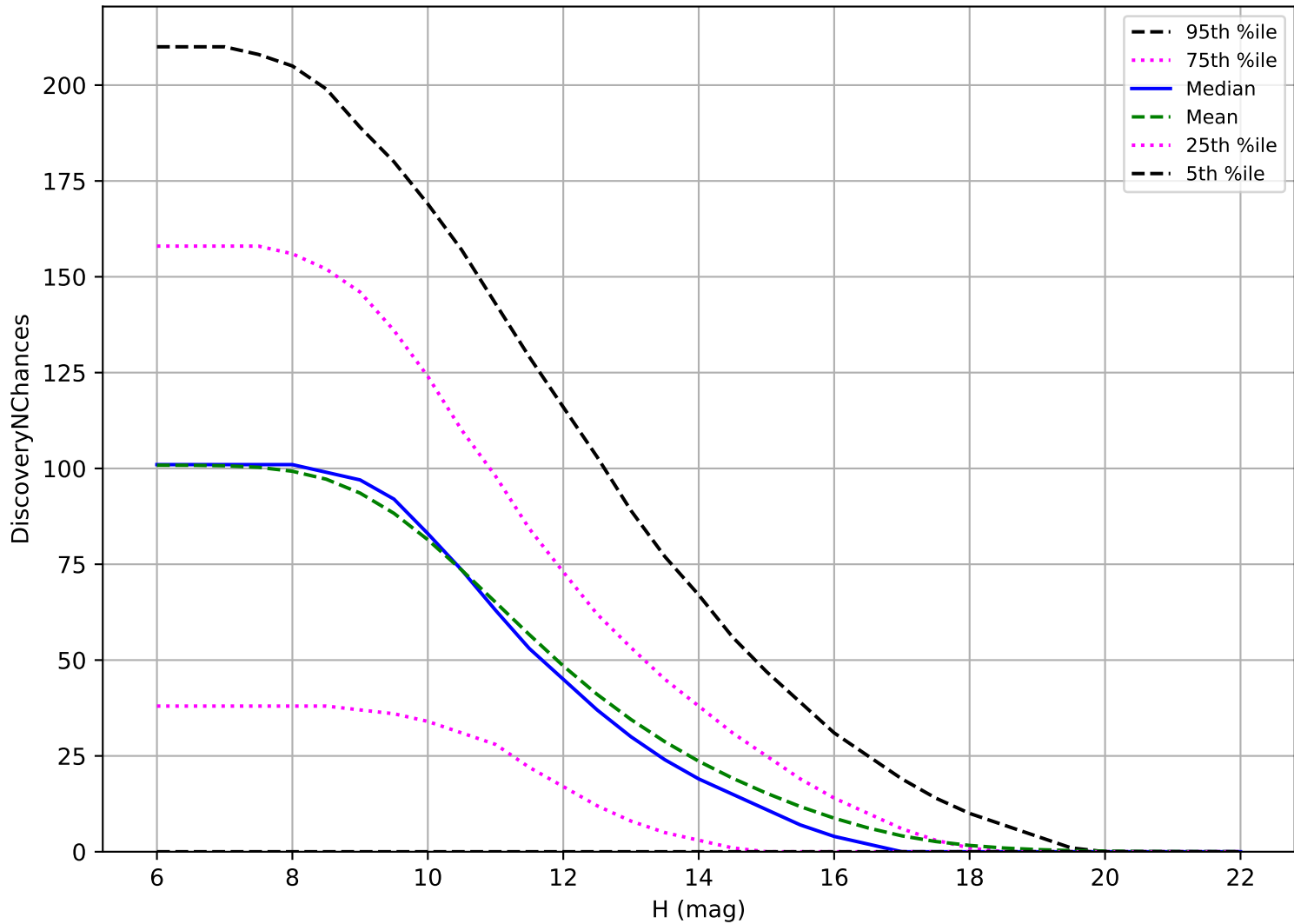
internal_u_expt38_nscale0.9v3.4_10yrs: OCC_r5 3 pairs in 15 nights detection loss
