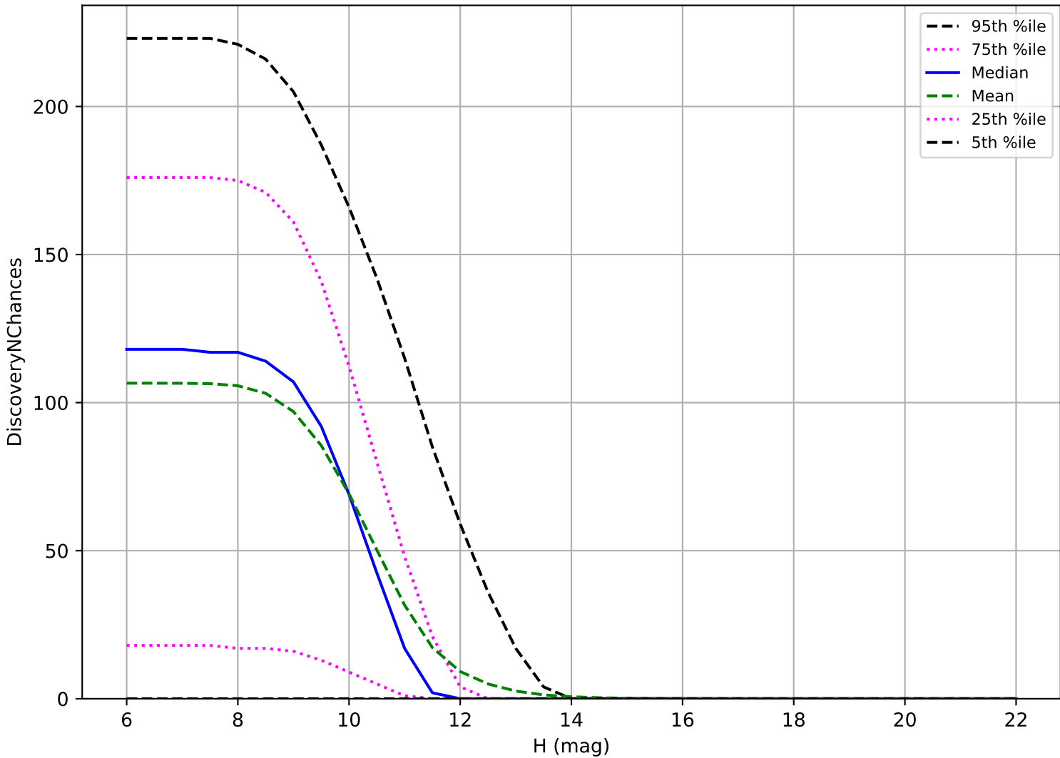
internal_u_expt38_nscale0.9v3.4_10yrs: OCC_r20 3 pairs in 15 nights detection loss
