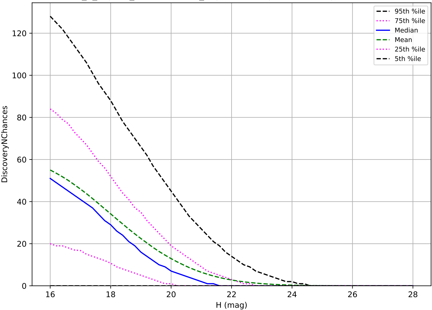
internal_u_expt38_nscale0.9v3.4_10yrs: NEO 3 pairs in 15 nights detection loss
