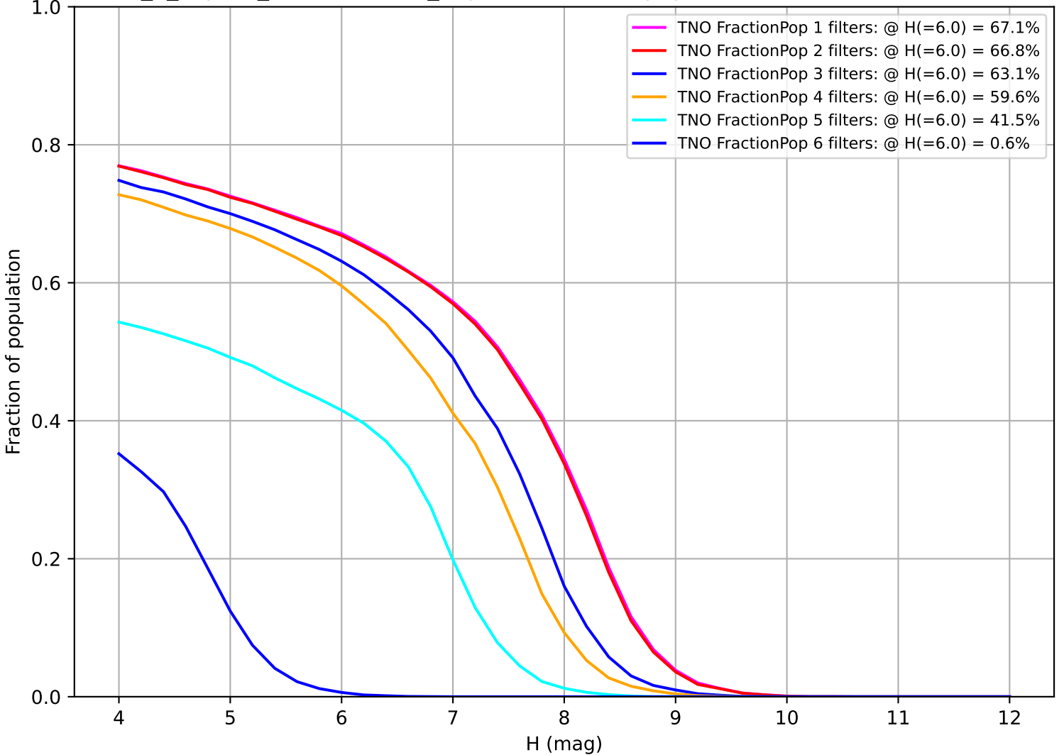
internal_u_expt38_nscale0.9v3.4_10yrs: Fraction of population with colors in X filters TNO
