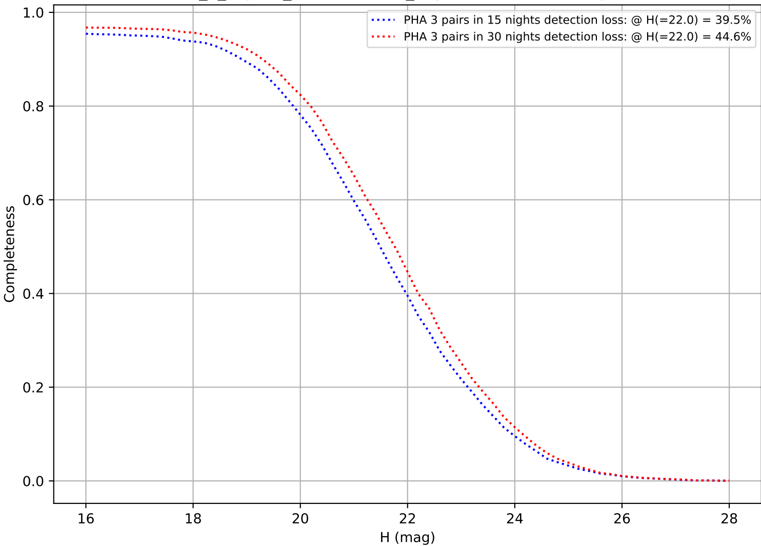
internal_u_expt38_nscale0.9v3.4_10yrs: DifferentialCompleteness
