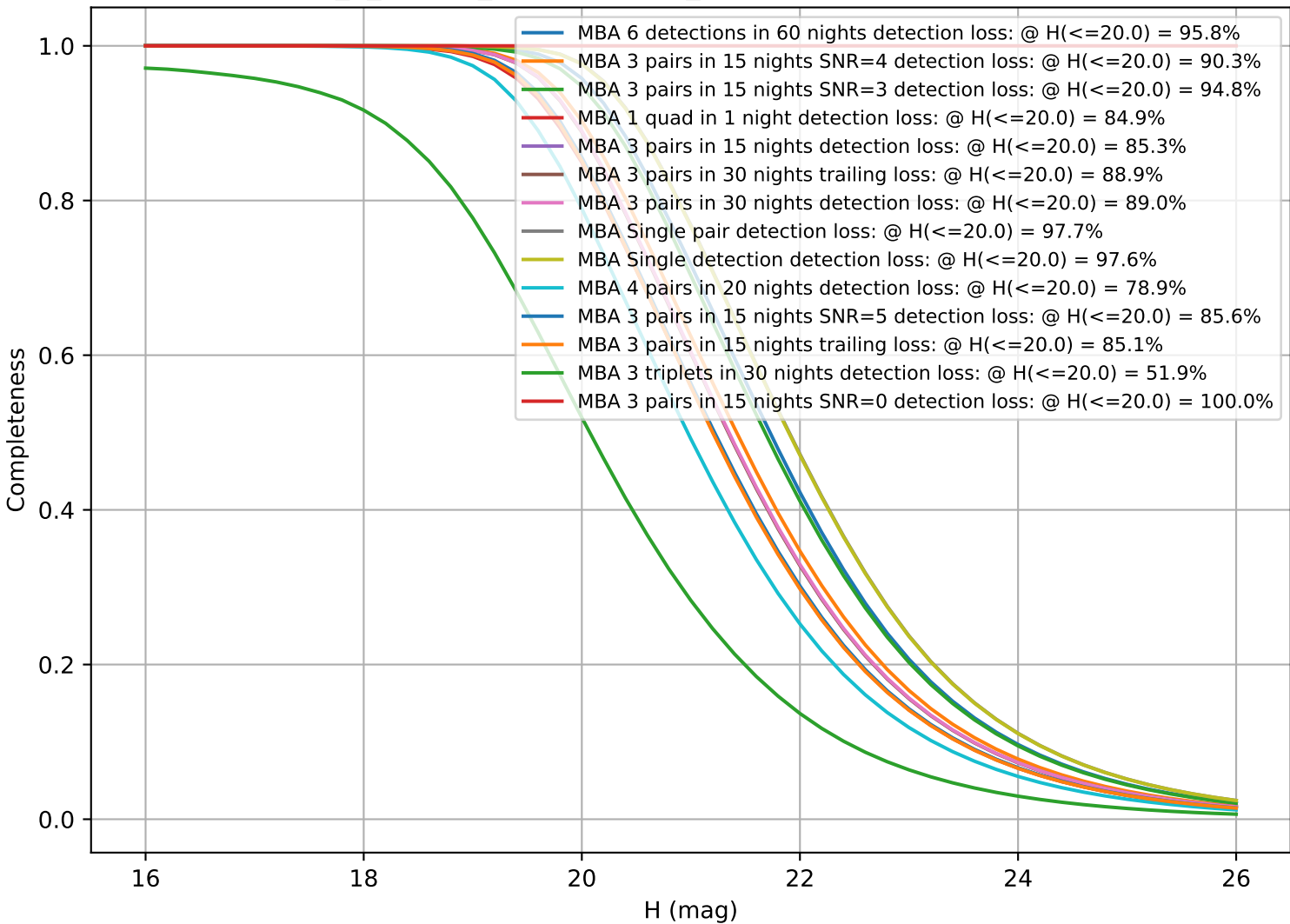
internal_u_expt38_nscale0.9v3.4_10yrs: CumulativeCompleteness
