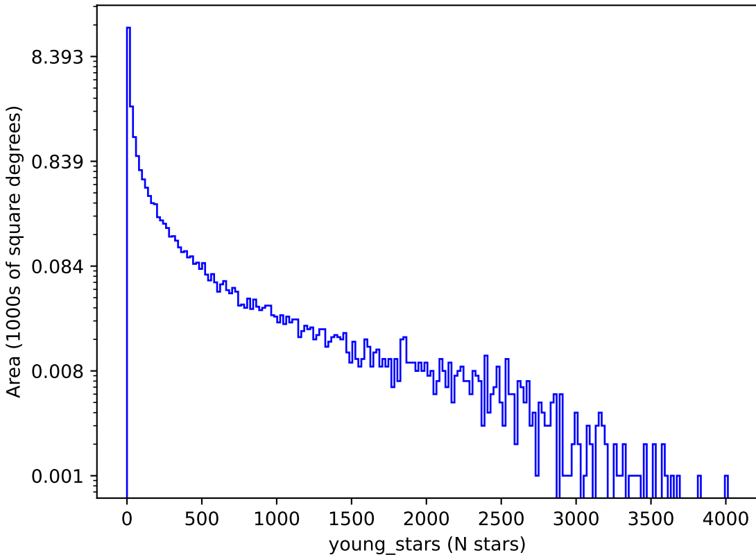
internal_u_expt38_nscale0.9v3.4_10yrs : young_stars
