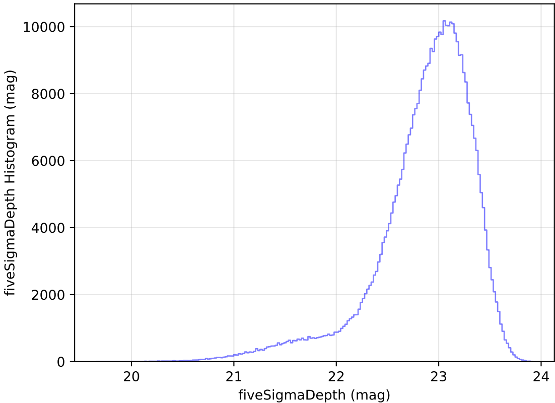
internal_u_expt38_nscale0.9v3.4_10yrs z: fiveSigmaDepth Histogram
