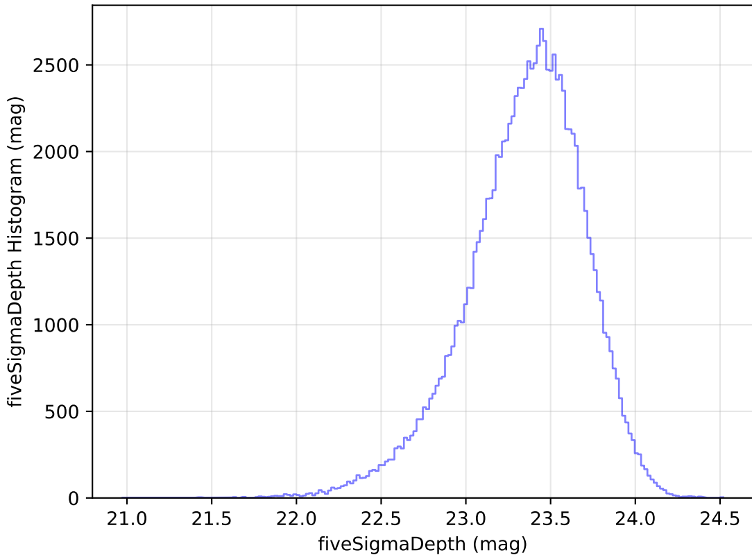
internal_u_expt38_nscale0.9v3.4_10yrs u: fiveSigmaDepth Histogram
