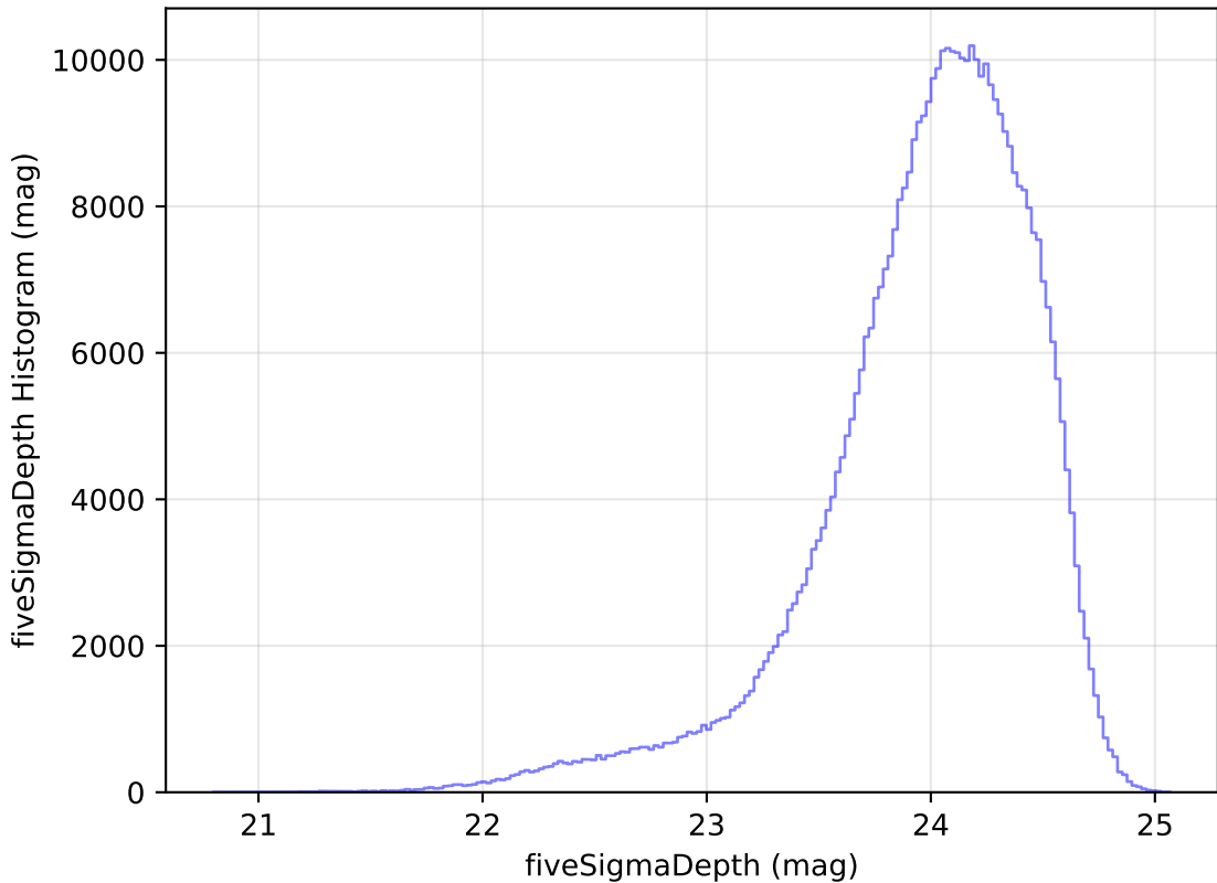
internal_u_expt38_nscale0.9v3.4_10yrs r: fiveSigmaDepth Histogram
