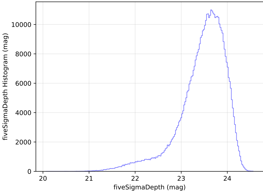
internal_u_expt38_nscale0.9v3.4_10yrs i: fiveSigmaDepth Histogram
