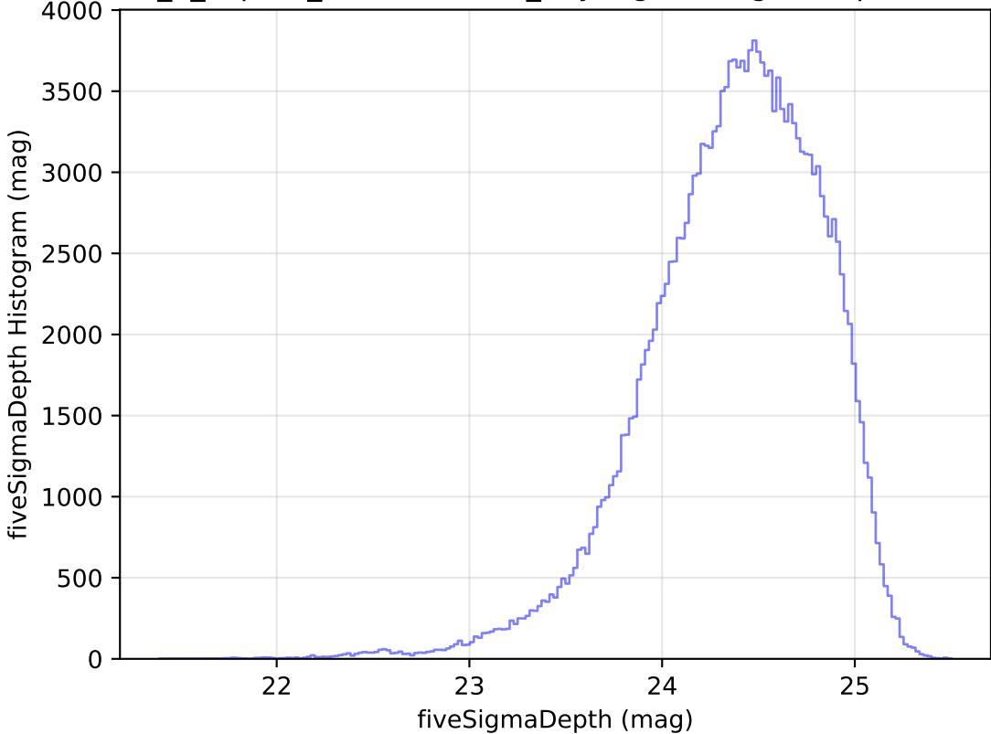
internal_u_expt38_nscale0.9v3.4_10yrs g: fiveSigmaDepth Histogram
