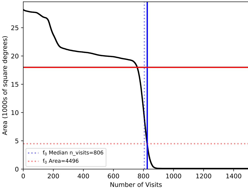
internal_u_expt38_nscale0.9v3.4_10yrs : fO
