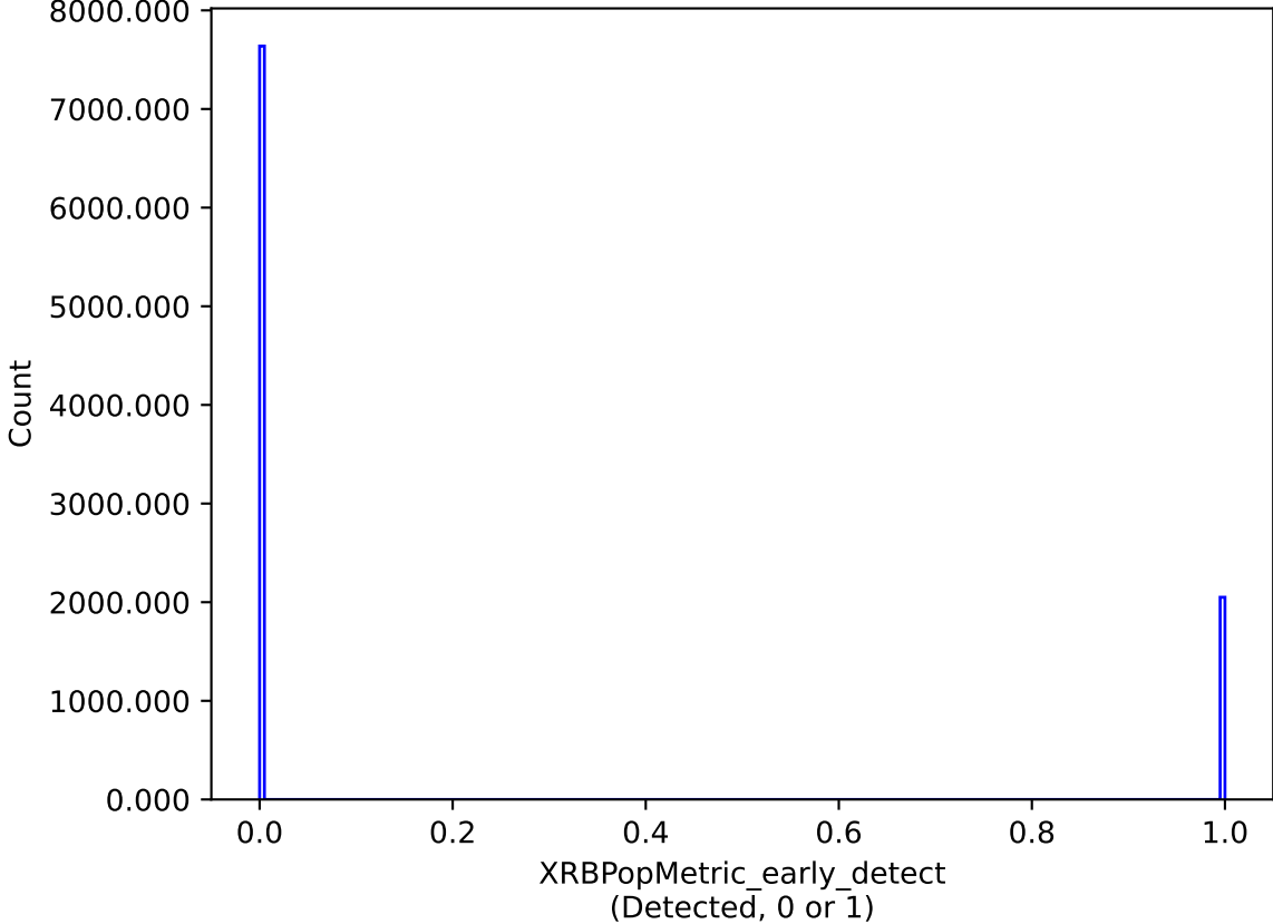
internal_u_expt38_nscale0.9v3.4_10yrs : XRBPoMetric_early_detect
