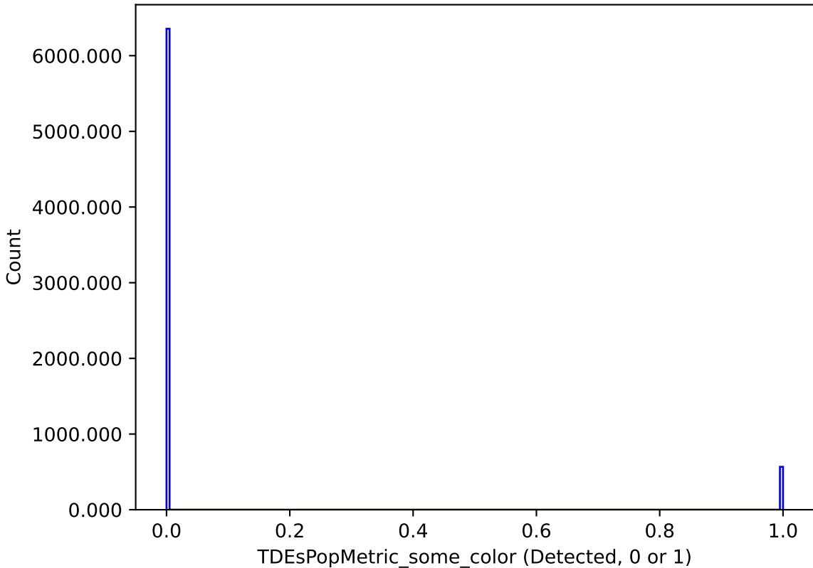
internal_u_expt38_nscale0.9v3.4_10yrs : TDEsPopMetric_some_color
