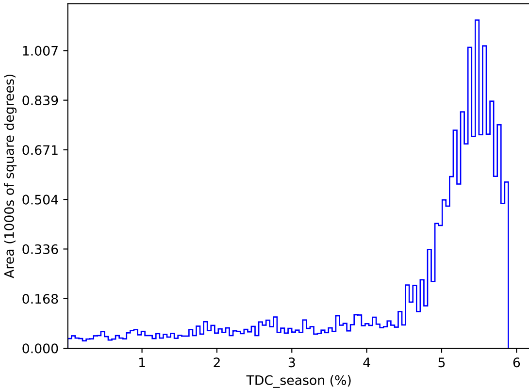
internal_u_expt38_nscale0.9v3.4_10yrs : TDC_season
