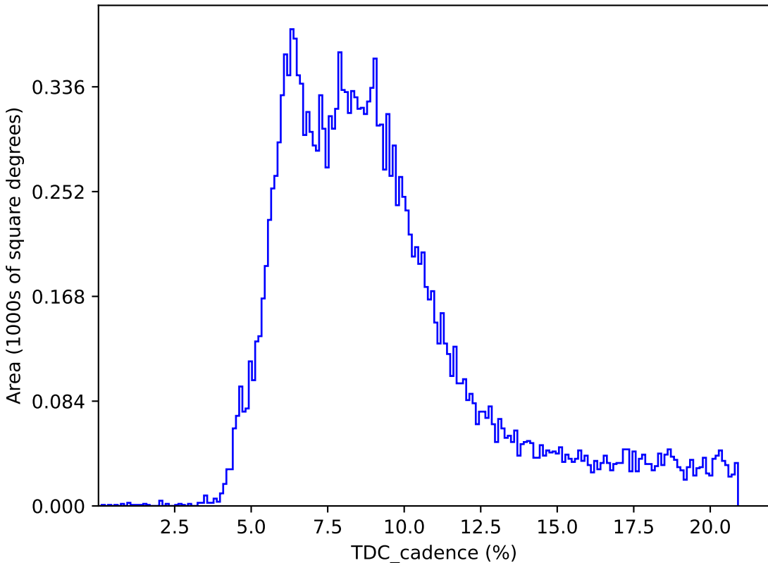
internal_u_expt38_nscale0.9v3.4_10yrs : TDC_cadence
