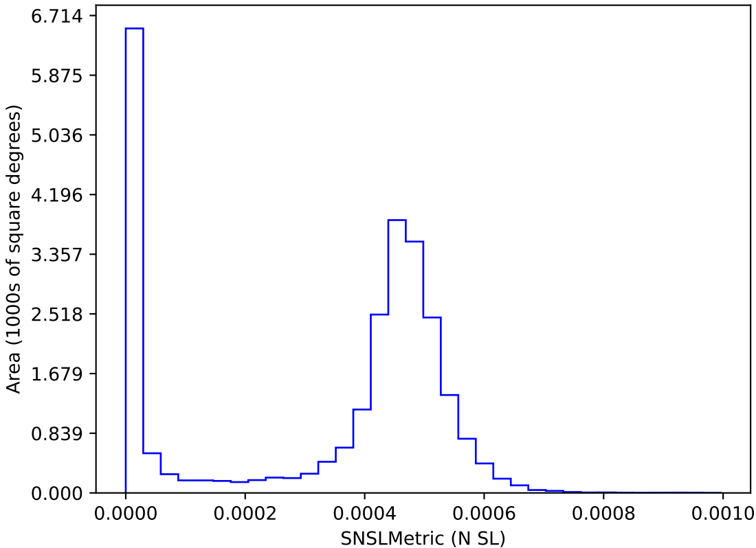
internal_u_expt38_nscale0.9v3.4_10yrs : SNSLMetric
