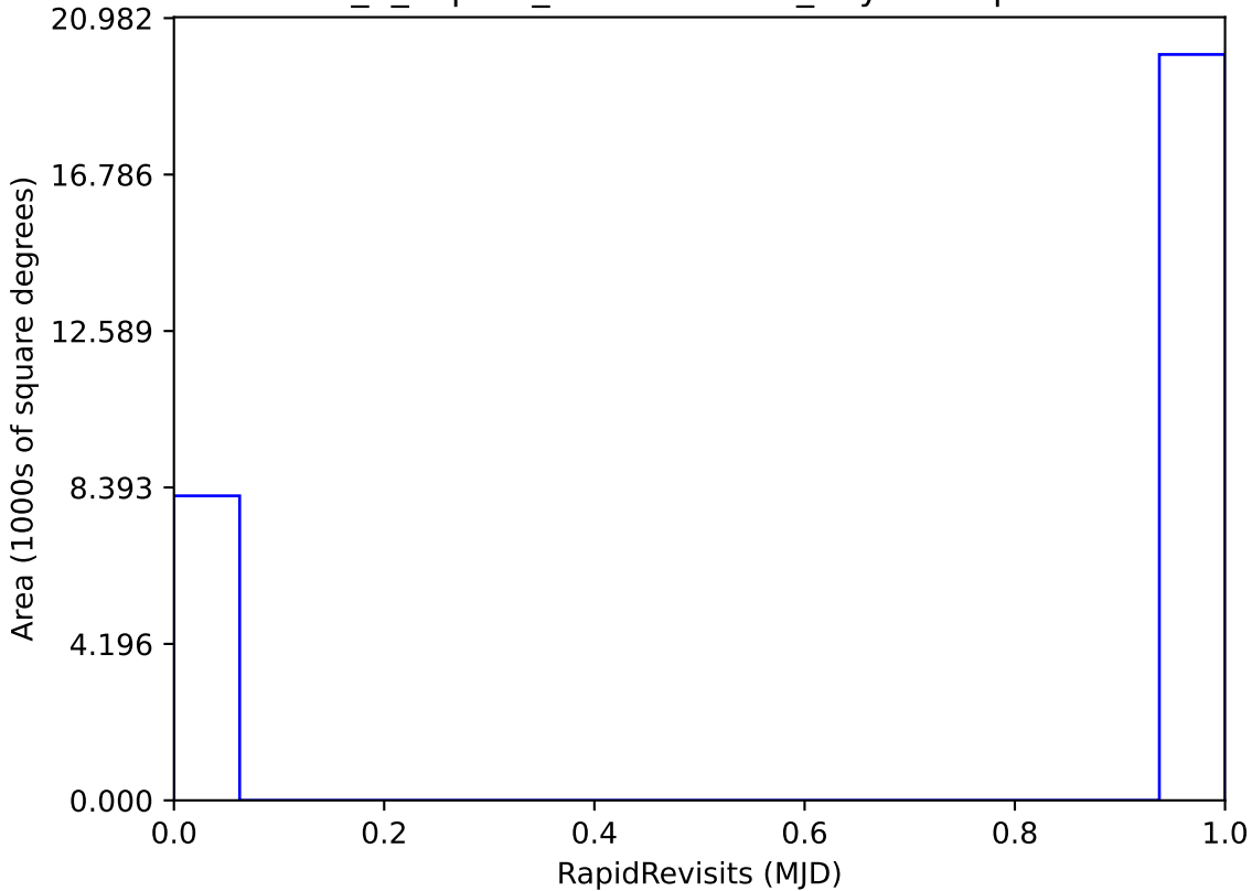
internal_u_expt38_nscale0.9v3.4_10yrs : RapidRevisits
