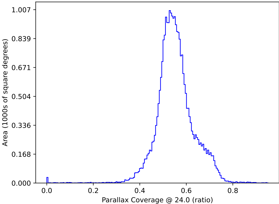
internal_u_expt38_nscale0.9v3.4_10yrs : Parallax Coverage @ 24.0
