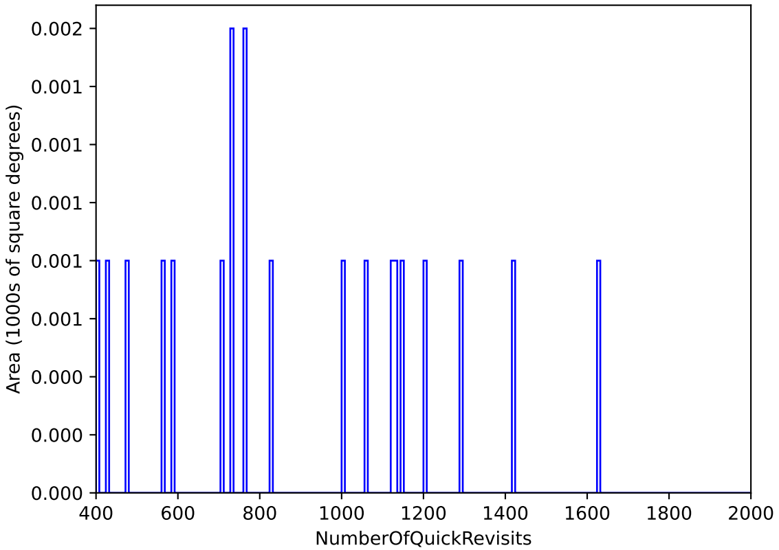
internal_u_expt38_nscale0.9v3.4_10yrs : NumberOfQuickRevisits
