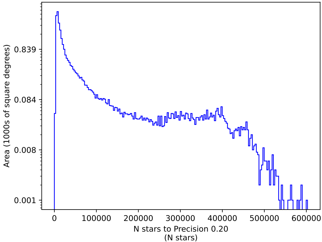
internal_u_expt38_nscale0.9v3.4_10yrs g: N stars to Precision 0.20
