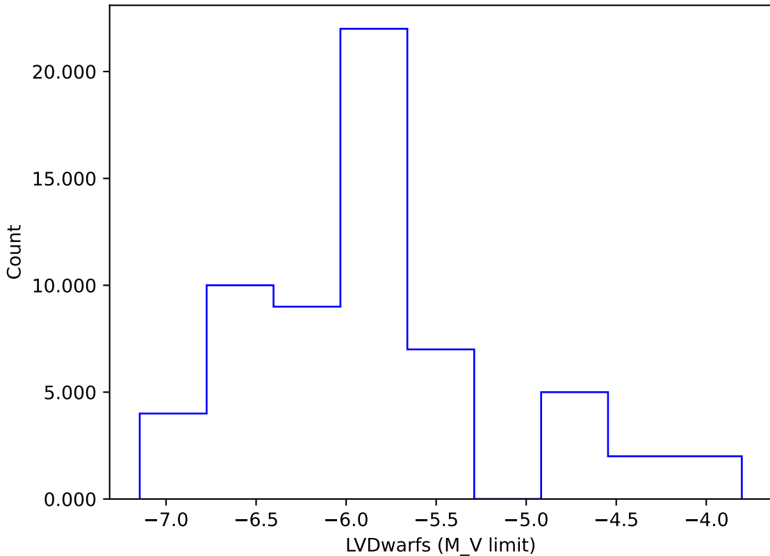
internal_u_expt38_nscale0.9v3.4_10yrs gi: LVDwarfs
