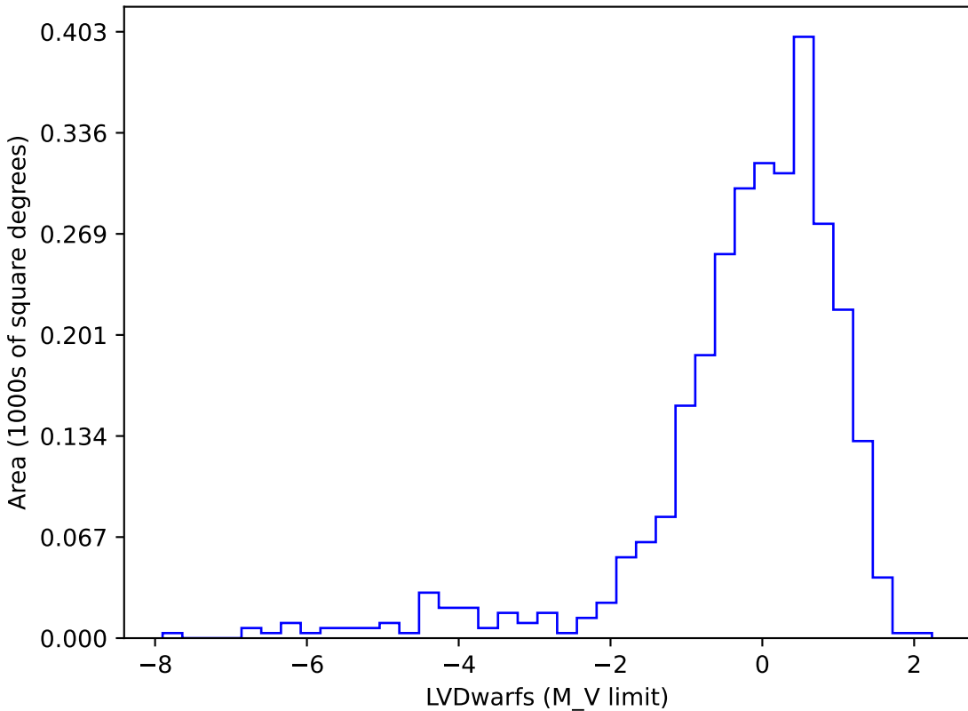
internal_u_expt38_nscale0.9v3.4_10yrs gi SCP: LVDwarfs
