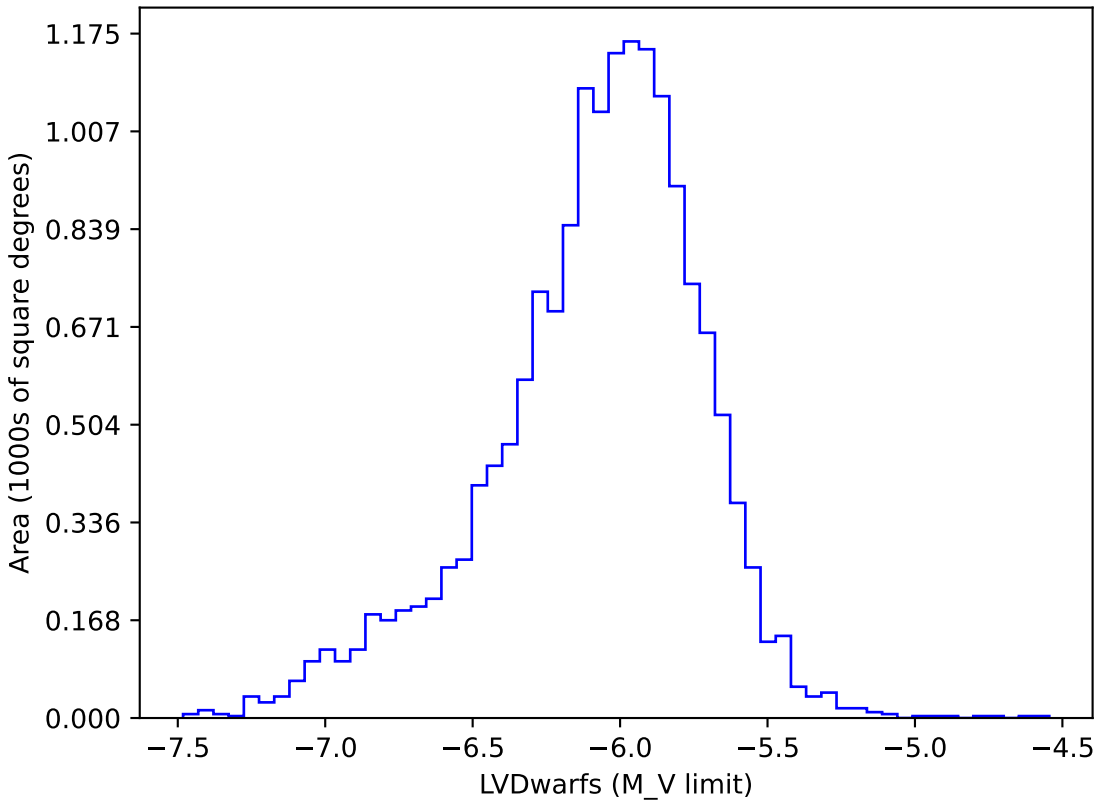
internal_u_expt38_nscale0.9v3.4_10yrs gi: LVDwarfs
