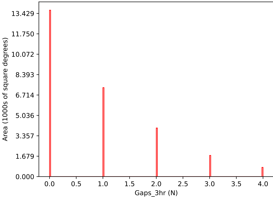
internal_u_expt38_nscale0.9v3.4_10yrs i band: Gaps_3hr
