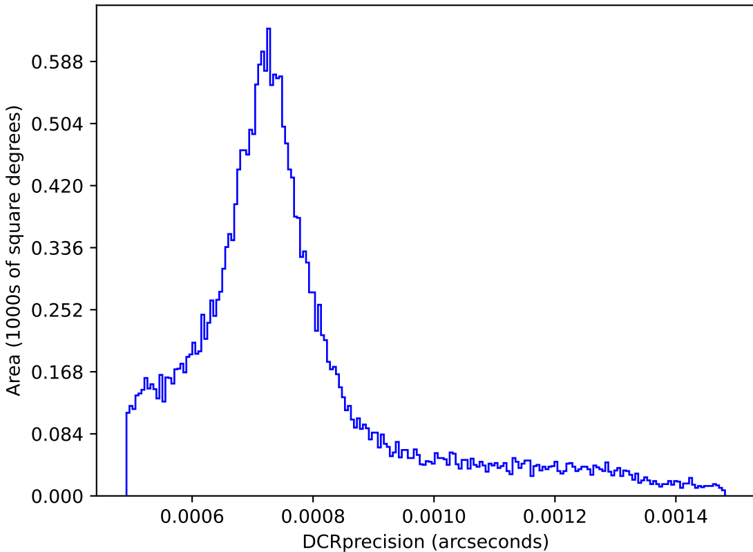
internal_u_expt38_nscale0.9v3.4_10yrs : DCRprecision
