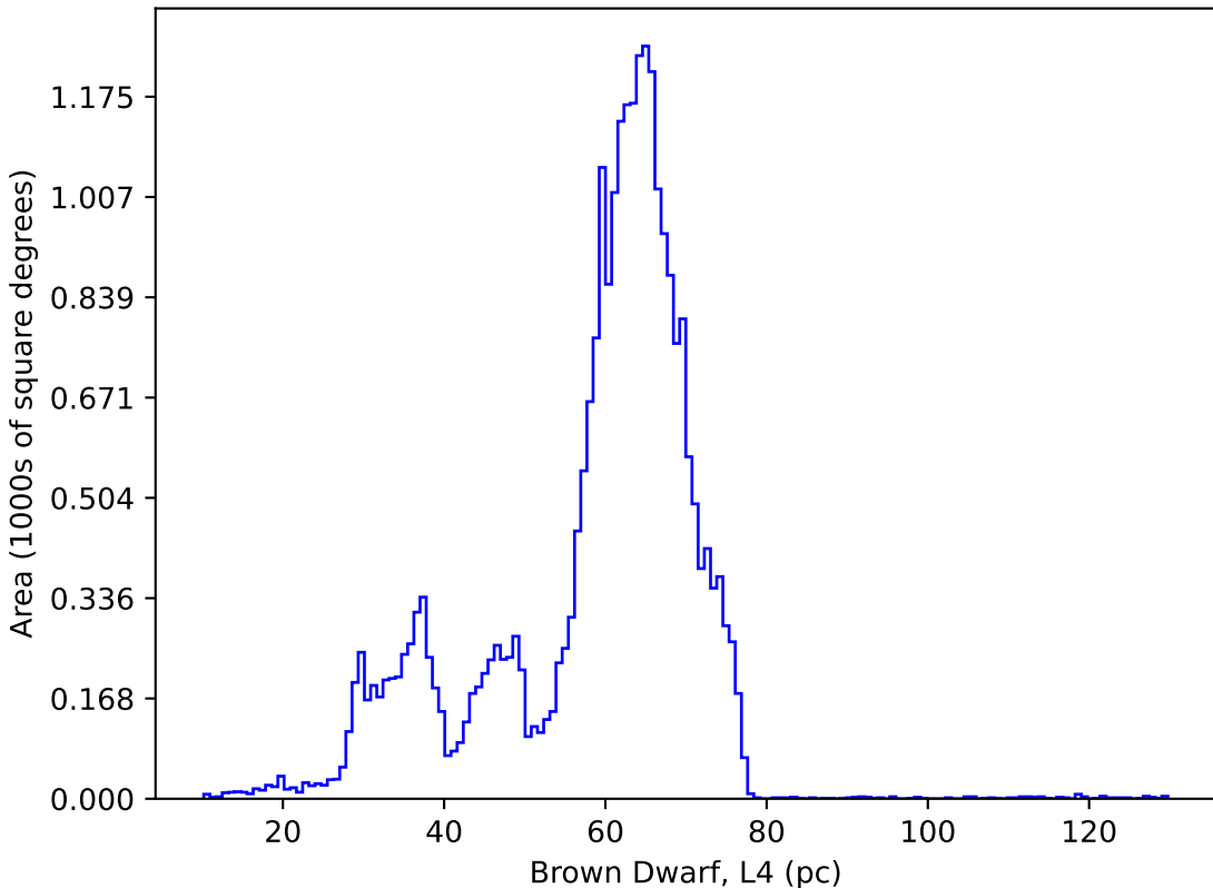
internal_u_expt38_nscale0.9v3.4_10yrs : Brown Dwarf, L4
