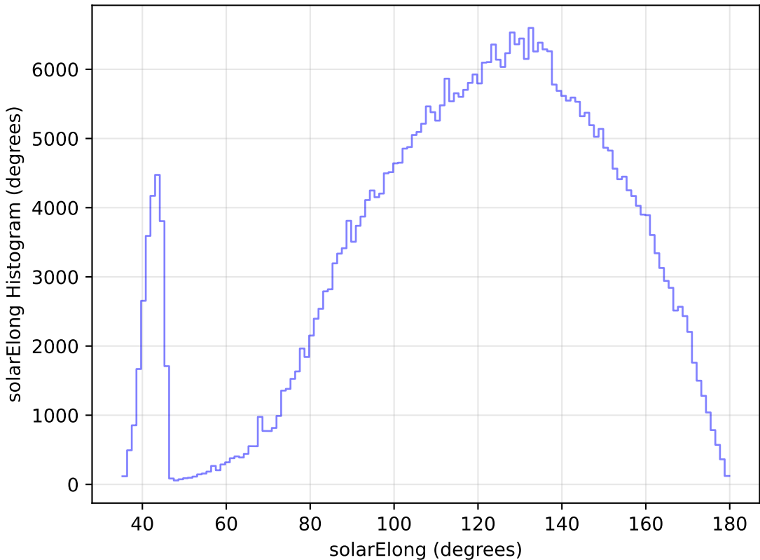
internal_u_expt38_nscale0.9v3.4_10yrs WFD z band: solarElong Histogram
