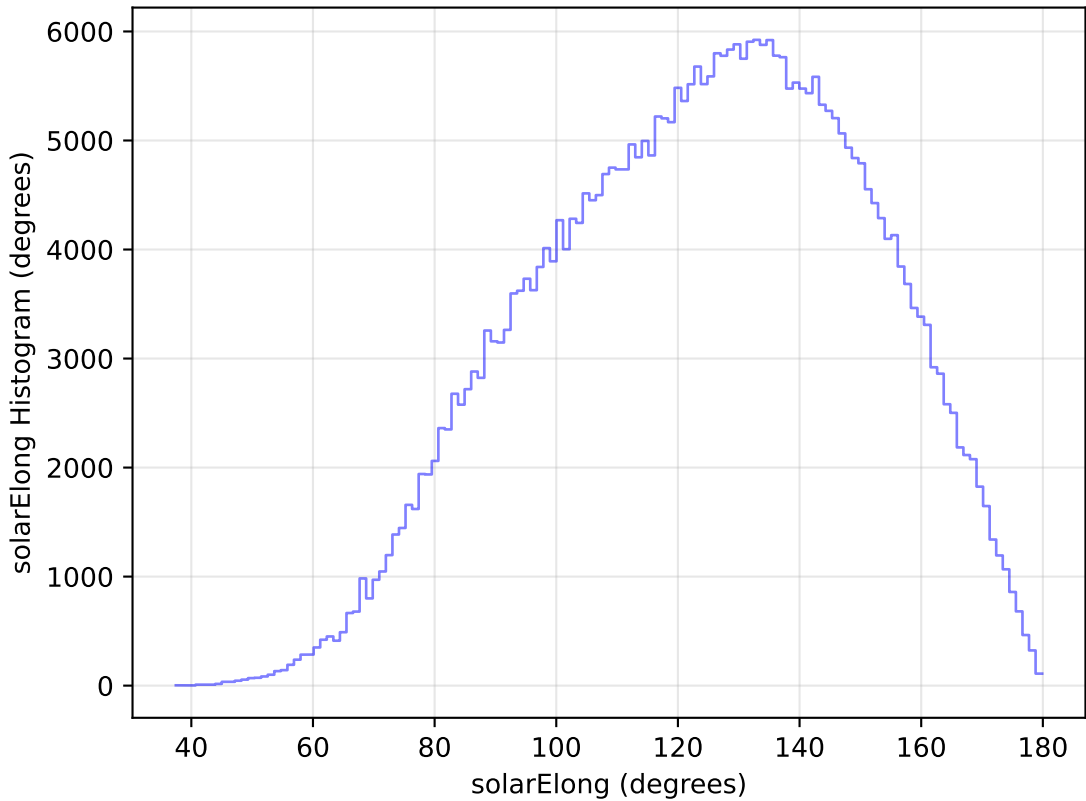
internal_u_expt38_nscale0.9v3.4_10yrs WFD y band: solarElong Histogram
