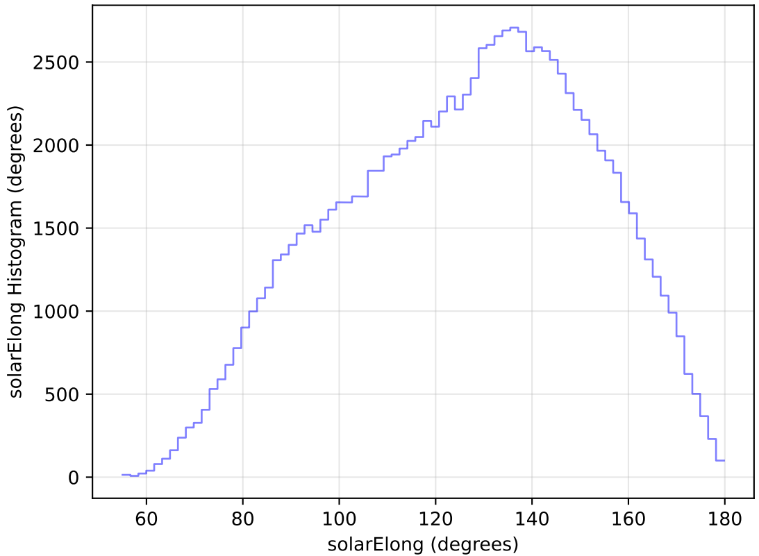
internal_u_expt38_nscale0.9v3.4_10yrs WFD u band: solarElong Histogram
