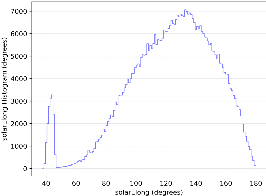
internal_u_expt38_nscale0.9v3.4_10yrs WFD r band: solarElong Histogram
