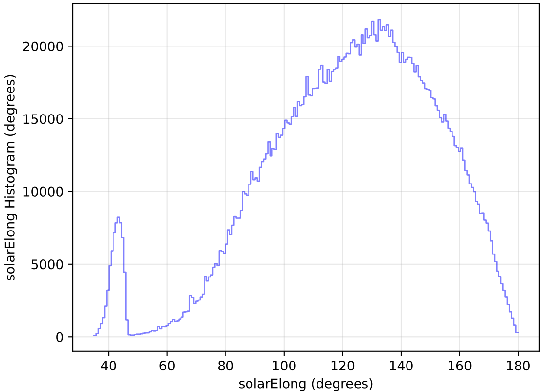
internal_u_expt38_nscale0.9v3.4_10yrs WFD all bands: solarElong Histogram
